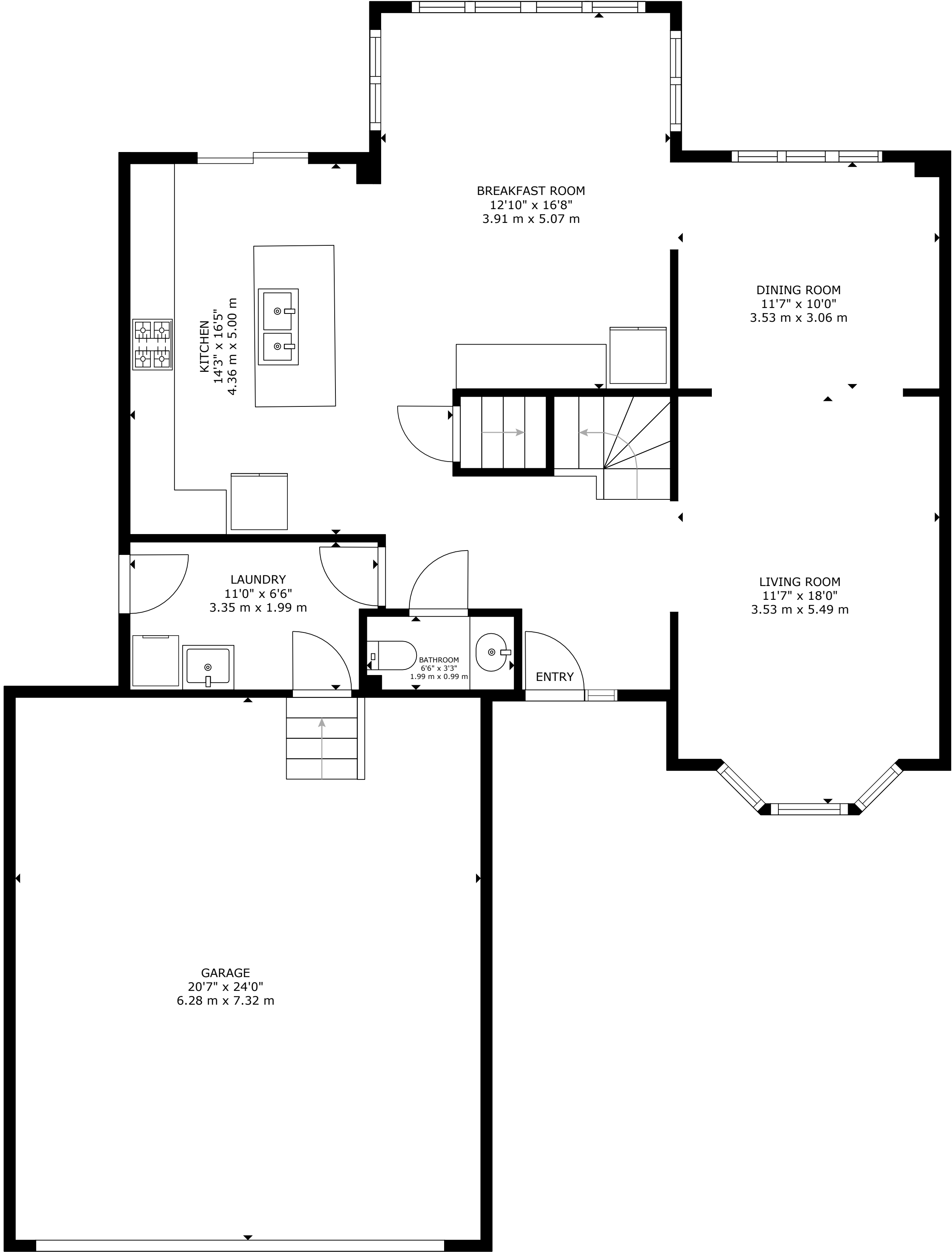
FLOOR 2
